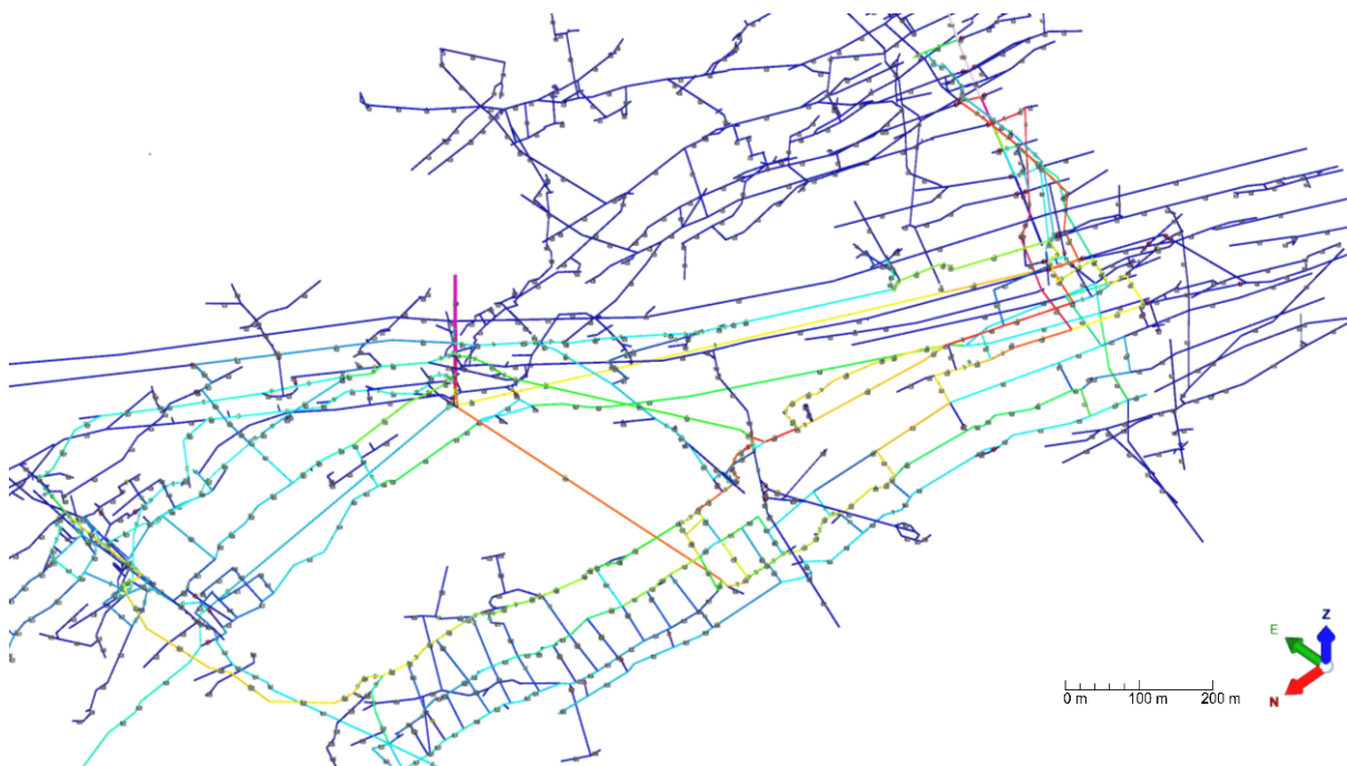
Figure 14 Ventilation model Reiche Zeche (Ventsim DESIGN)
