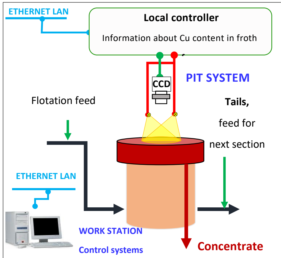
Figure 18 Overall concept and role of PIT System in processing of copper ore
