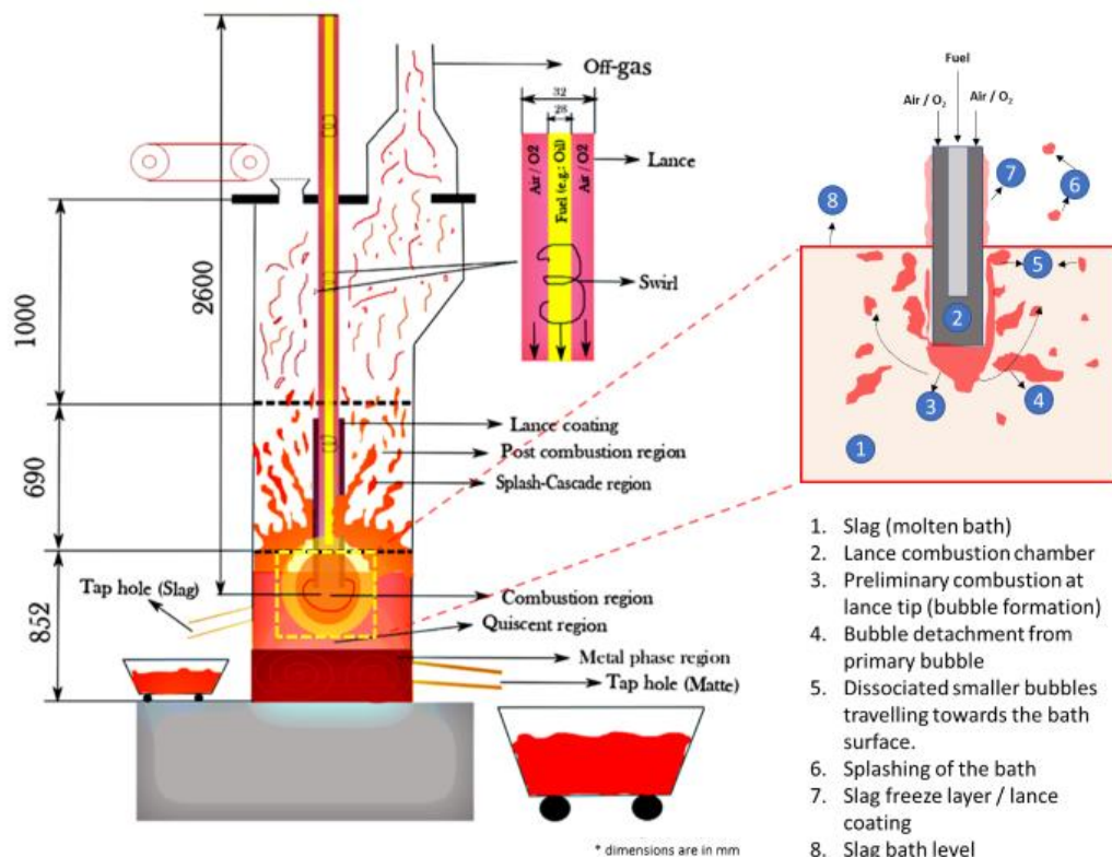
Figure 15 Schematic illustration of the TSL smelter featuring its components, mechanism and dimensions of the pilot-TSL at TU Bergakademie Freiberg
