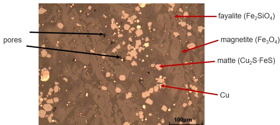
Figure 17 Typical composition of a fayalitic slag from the primary copper process
