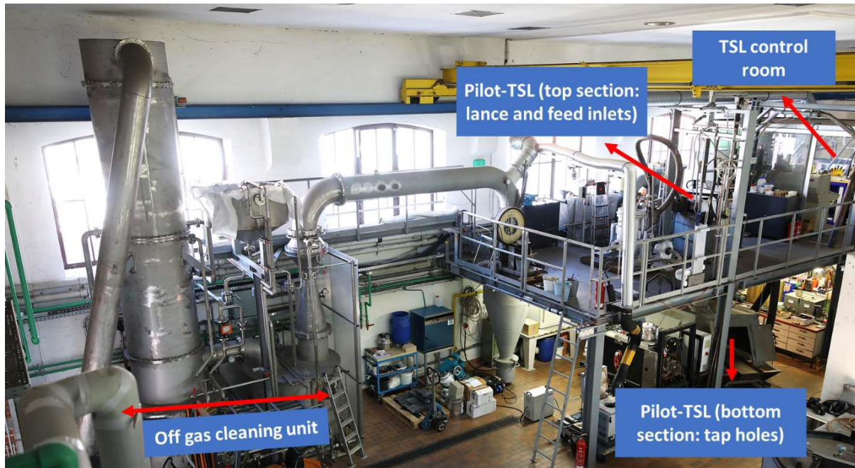
Figure 16 Photo of the TSL Smelter with the off-gas cleaning unit in the furnace hall of the Institute of Nonferrous Metallurgy at TU Bergakademie Freiberg
