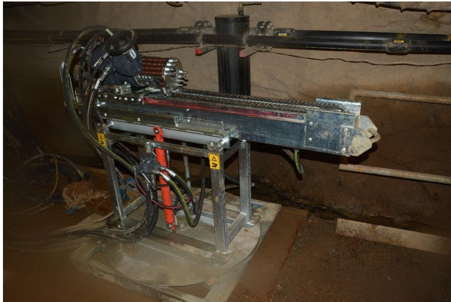
Figure 9 Drilling Machine Sandvik DE110 (2015)
